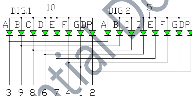
OPS-D3910SPG (Common Anode)
