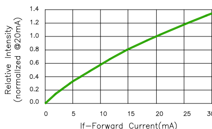
Fig.2—Relative Luminous Intensity vs. Forward Current
