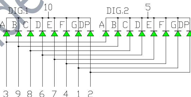
OPS-D3911SPG (Common Cathode)
