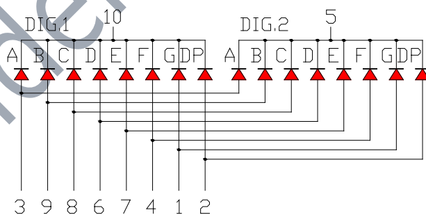
OPS-D3911SE (Common Cathode)
