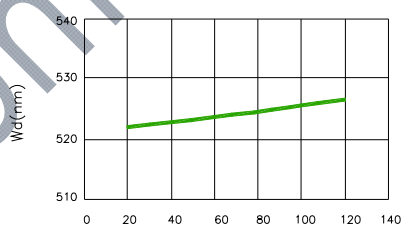
Fig. 6-Dominant Wavelength(@20mA) VS. Ambient Temperature
