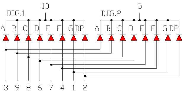
OPS-D3921LE-2-STT(R)-1.0-G(B)W (Common Cathode)
