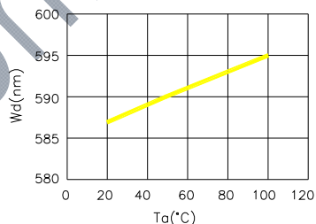
Fig.6-Dominant Wavelength(@20mA) VS. Ambient Temperature
