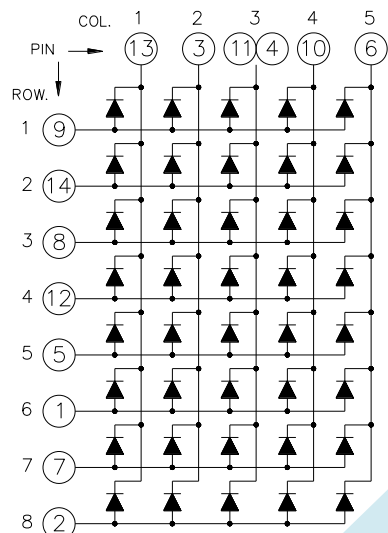
OPD-M35811 Anode Row Cathode Column
