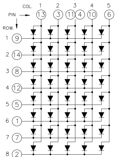
OPD-M35810 Anode Column Cathode Row
