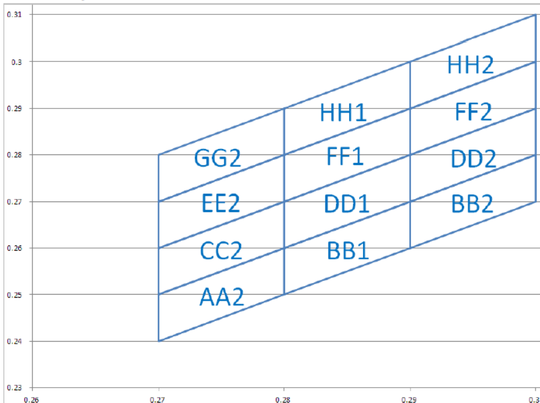
■ Chromaticity Coordinate
