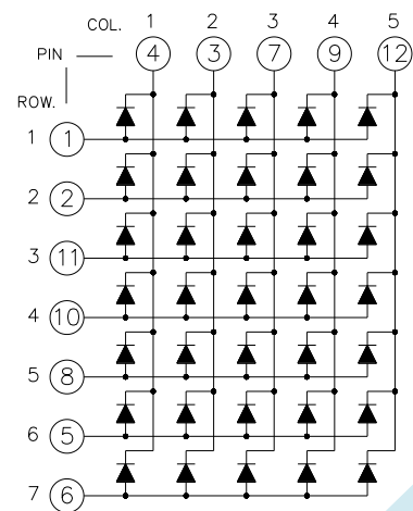
OPD-M25713 Anode Row Cathode Column
