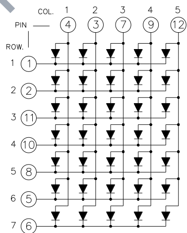
OPD-M25712 Anode Column Cathode Row
