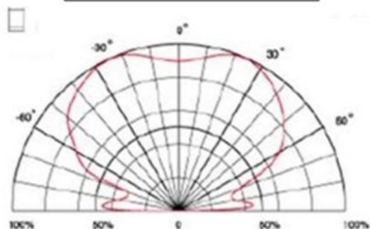
Directive Characteristics
