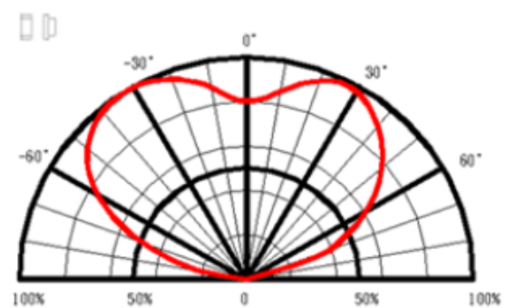
Directive Characteristics
