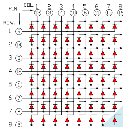
OPD-M48831 CATHODE COLUMN, ANODE ROW
