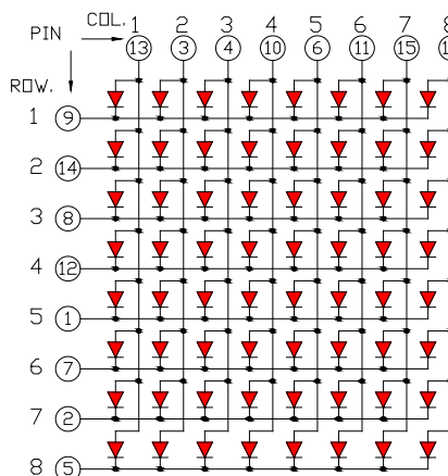
OPD-M48830 ANODE COLUMN, CATHODE ROW
