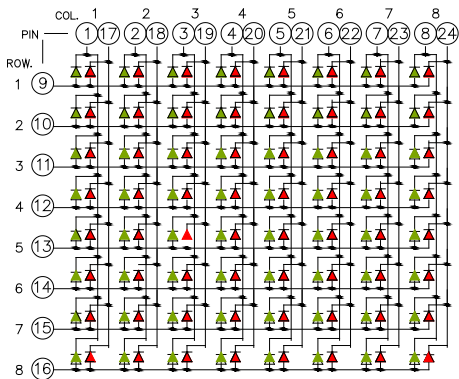
OPD-M288A1 Anode Row Cathode Column
