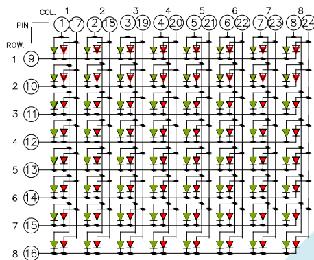
OPD-M288A0 Anode Column Cathode Row
