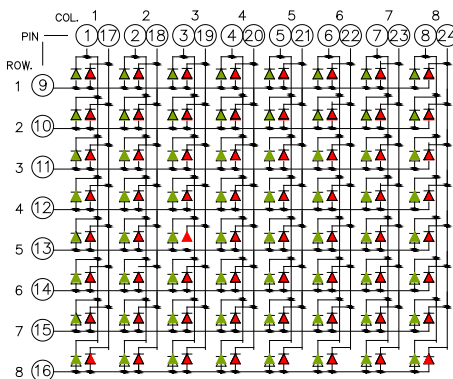
OPD-M288A1 Anode Row Cathode Column
