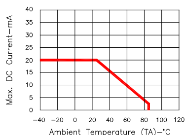
Fig.7—Max. Allowable DC Current VS. Ambient Temperature
