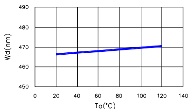
Fig.6-Dominant Wavelength(@20mA) VS. Ambient Temperature
