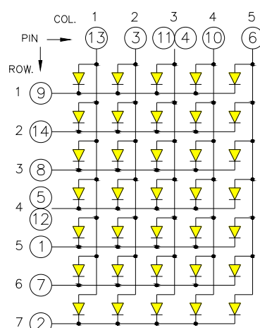
OPD-M35720 Anode Column Cathode Row
