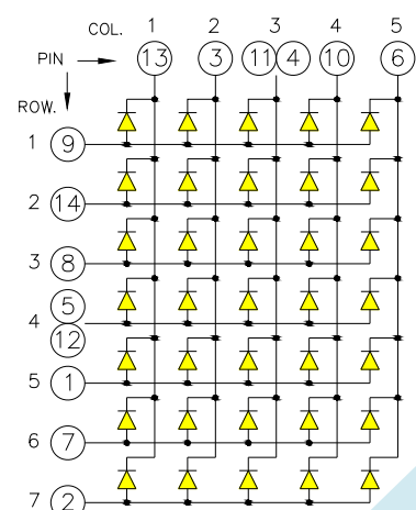
OPD-M35721 Anode Row Cathode Column
