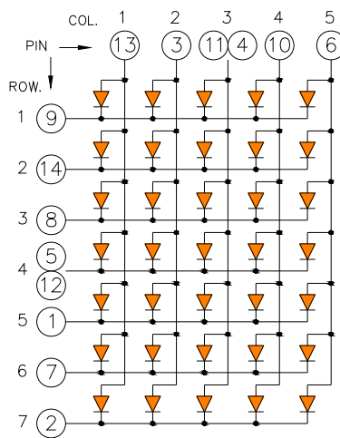
OPD-M35710 Anode Column Cathode Row
