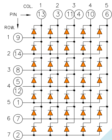
OPD-M35711 Anode Row Cathode Column
