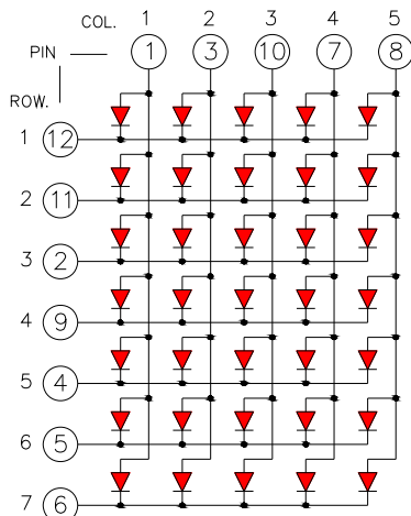
OPD-M25710 Anode Column Cathode Row
