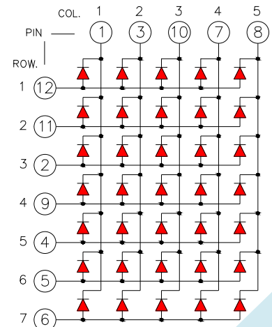
OPD-M25711 Anode Row Cathode Column
